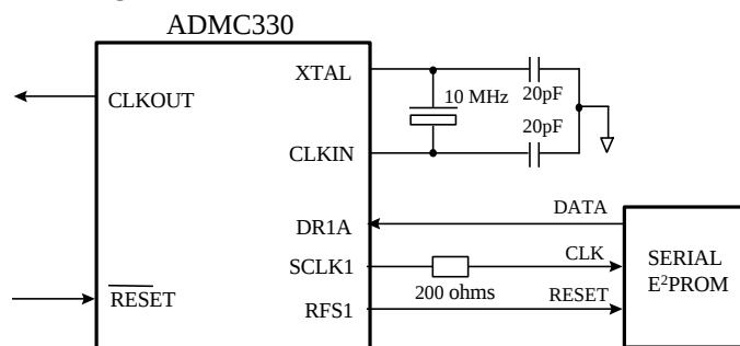
Figure 3: Connection of serial memory (ROM or E 2 PROM) and crystal to the ADMC330.
