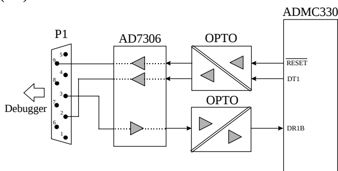
Figure 2: Functional Block Diagram of UART Interface to Motion Control Debugger of ADMC330 PROCESSOR BOARD.
