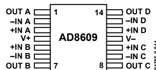
Figure 4. 14-Lead TSSOP (RU Suffix)
