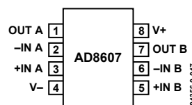
Figure 3. 8-Lead SOIC (R Suffix)
