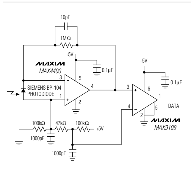
Figure 3. Battery-Operated Infrared Data Link Consumes Only 760μA
