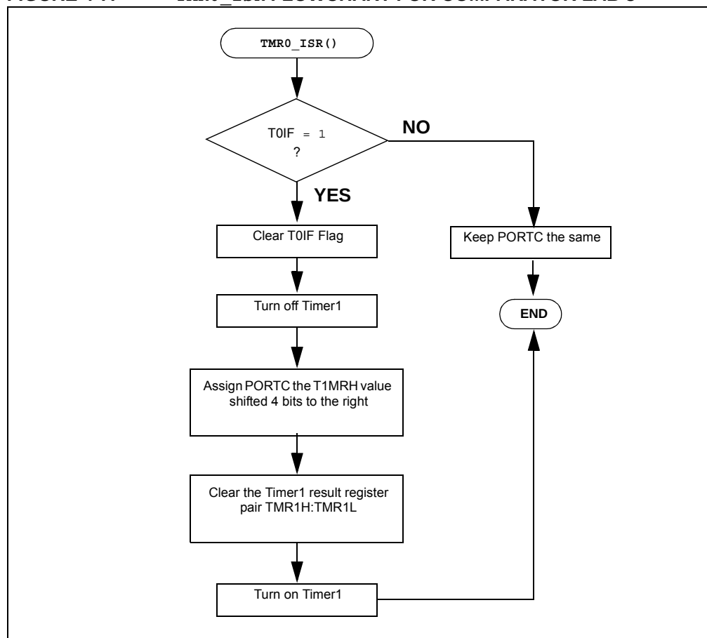
FIGURE 4-7: TMR0_ISR FLOWCHART FOR COMPARATOR LAB 3
