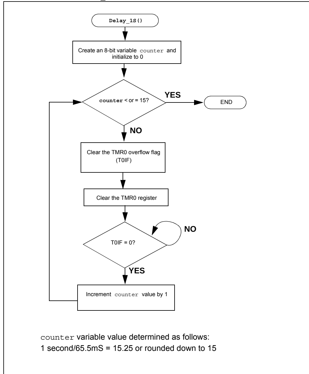
FIGURE 3-14: DELAY_1S () USING TMR0
