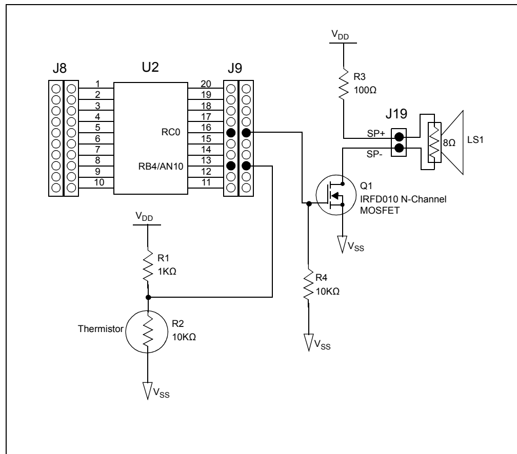
FIGURE 5-5: SCHEMATIC FOR ADC LAB 2
