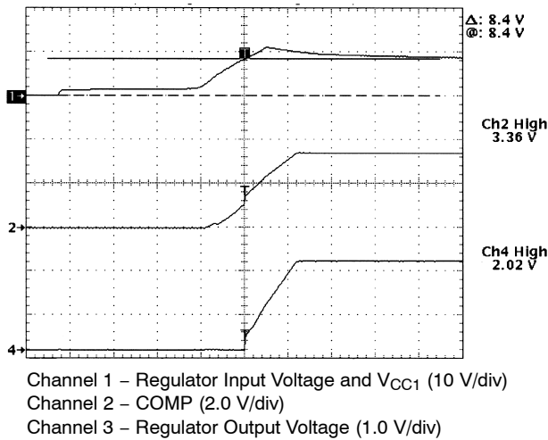
Figure 10. Normal Startup (5.0 ms/div)
