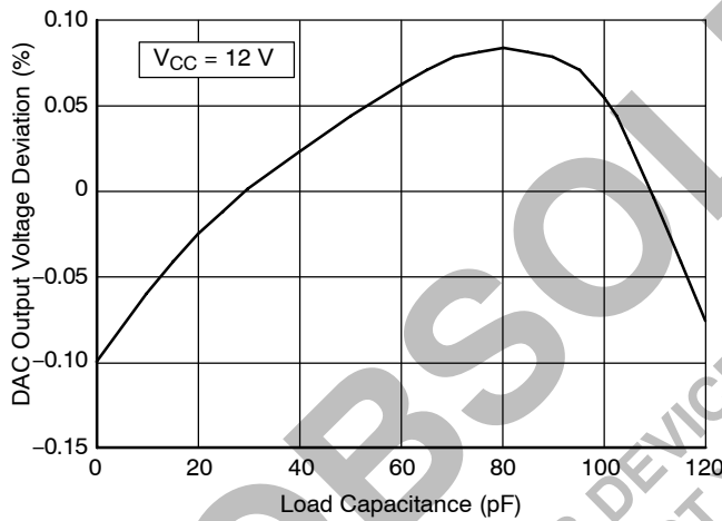
Figure 5. DAC Output Voltage vs. Load Capacitance, DAC Code = 00001
