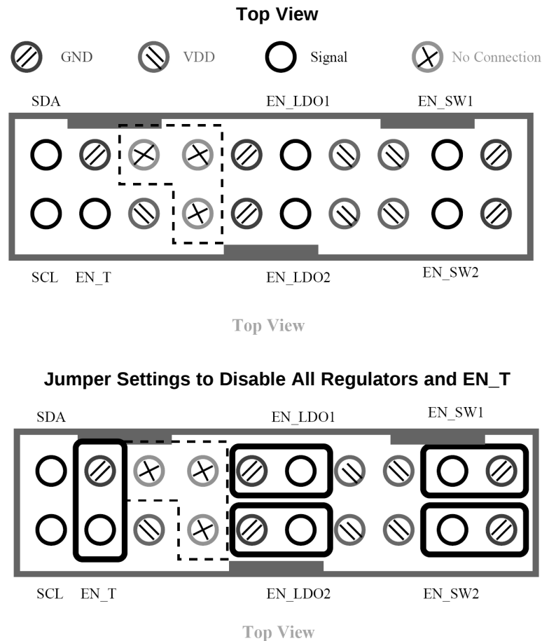
Figure 10. Header Connector
