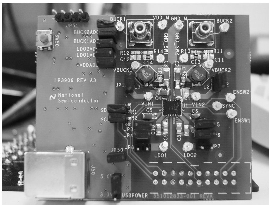
Figure 1. Evaluation Board
