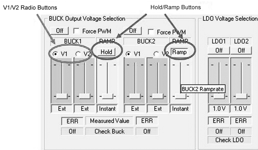
Figure 7. Regulator Output Voltage Selection Interface
