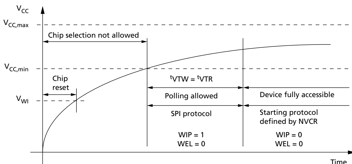
Figure 38: Power-Up Timing
