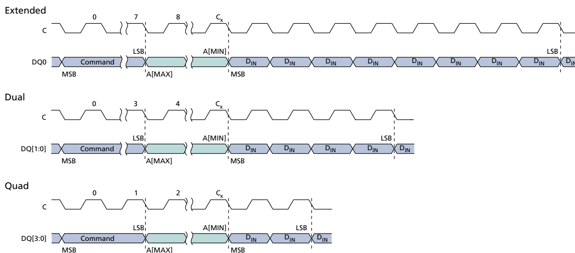
Figure 36: PROGRAM OTP Command
