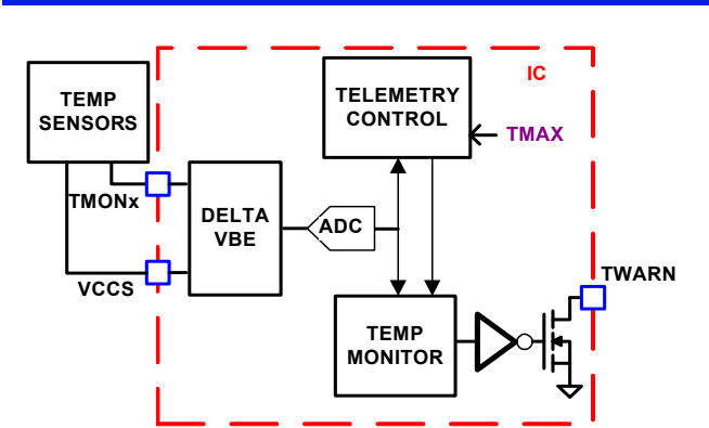
FIGURE 23. BLOCK DIAGRAM OF THERMAL MONITORING FUNCTION
