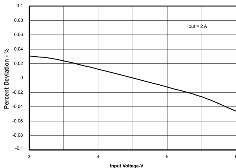
Figure 4. TPS54418EVM-375 Line Regulation
