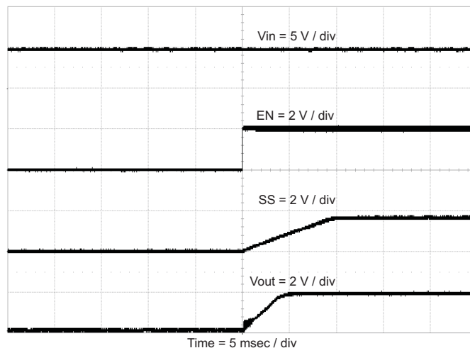
Figure 10. TPS54418EVM-375 Start-up Relative to Enable
