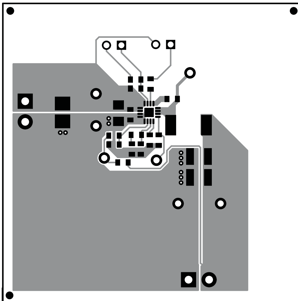
Figure 11. TPS54418EVM-375 Top-Side Layout
