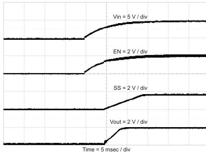
Figure 9. TPS54418EVM-375 Start-Up Relative to V_{IN}
