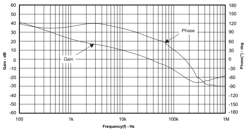
Figure 6. TPS54418EVM-375 Loop Response
