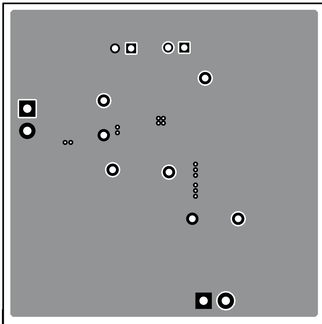
Figure 14. TPS54418EVM-375 Layout 3
