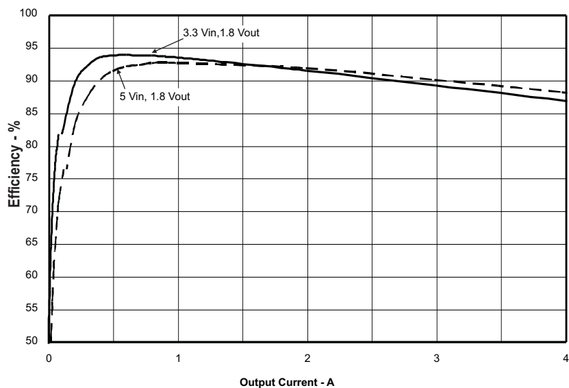
Figure 1. TPS54418EVM-375 Efficiency
