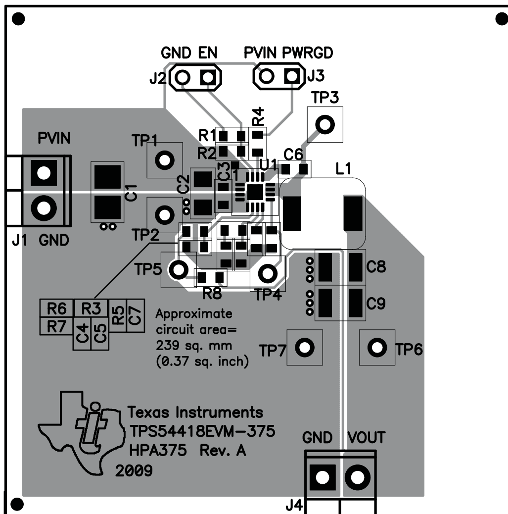
Figure 15. TPS54418EVM-375 Top-Side Assembly
