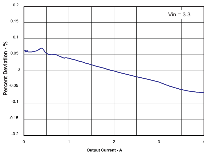
Figure 3. TPS54418EVM-375 Load Regulation
