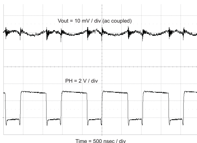
Figure 7. TPS54418EVM-375 Output Ripple
