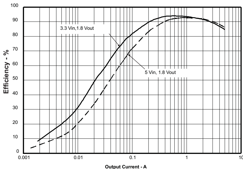
Figure 2. TPS54418EVM-375 Low Current Efficiency
