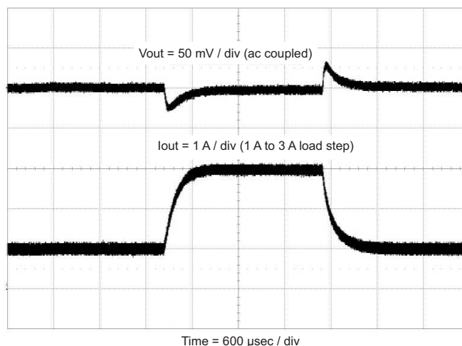
Figure 5. TPS54418EVM-375 Transient Response
