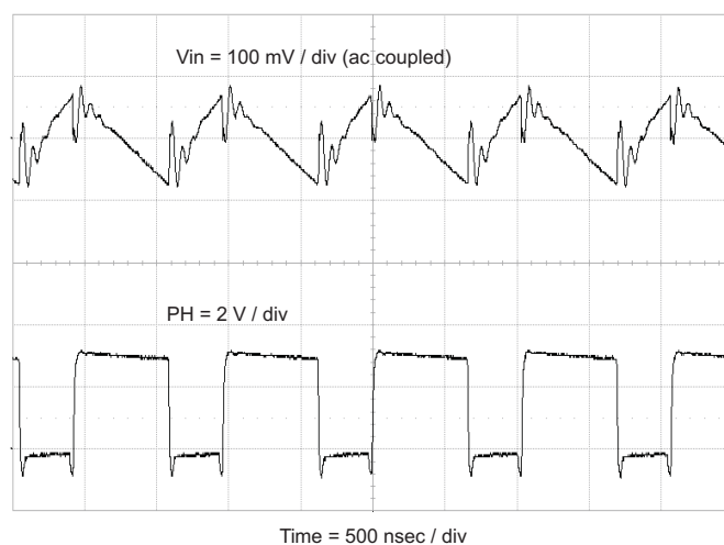
Figure 8. TPS54418EVM-375 Input Ripple
