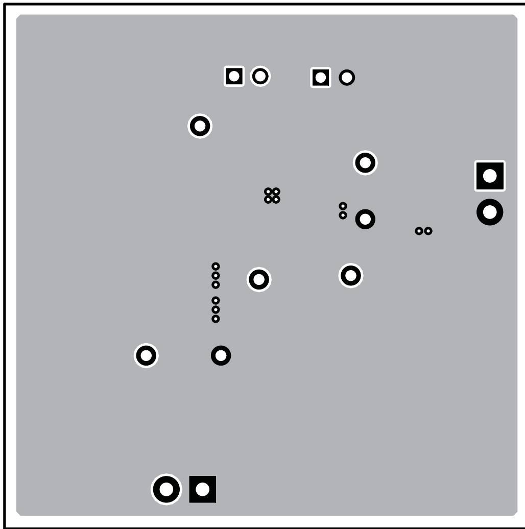
Figure 12. TPS54418EVM-375 Bottom-Side Layout
