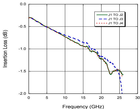
Insertion Loss
