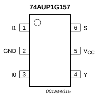
Fig 5. Pin configuration SOT363 (SC-88)
