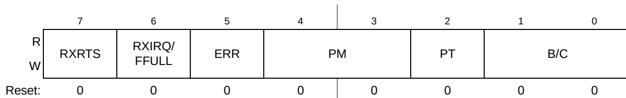
Figure 23-3. UART Mode Registers 1 (UMR1n)
