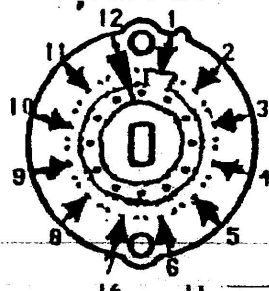
WAFER 1 REAR
