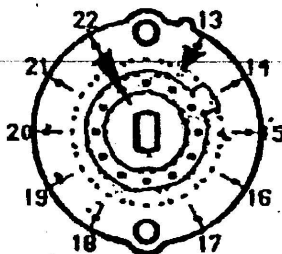
WAFER 1 FRONT/REAR
