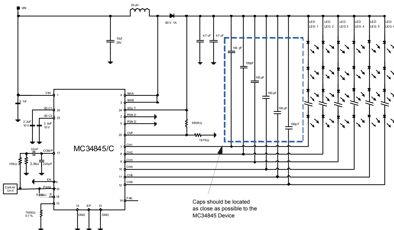
Figure 10. Typical Application Circuit for Single Wire Control, f_s = 600 \text{ KHz} ( V_{IN} = 9.0 \text{ V} , I_{LED}/\text{channel} = 20 \text{ mA/channel} , 10 LEDs/channel, OVP = 35 \text{ V} , V_{PWM} = 3.3 \text{ V} )
