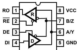
ISL32492E, ISL32495E, ISL32498E (8 LD MSOP, 8 LD SOIC) TOP VIEW
