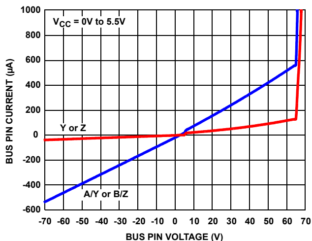
FIGURE 15. BUS PIN CURRENT vs BUS PIN VOLTAGE
