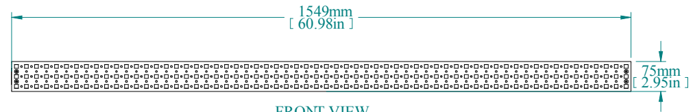
FRONT VIEW
