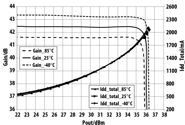
Figure 22. Over-temperature Gain, I_{dd\_total} vs. P_{out} @ 2.36GHz V_{dd}=V_{ddBias}=5.0 V operating voltage
