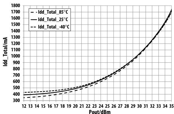
Figure 24. Over-temperature I_{dd\_total} vs. P_{out} @ 2.35 GHz V_{dd}=V_{ddBias}=5.0 V operating voltage
