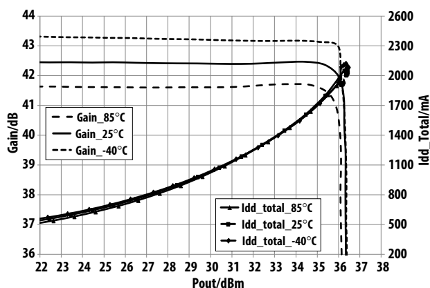
Figure 21. Over-temperature Gain, I_{dd\_total} vs. P_{out} @ 2.35 GHz V_{dd}=V_{ddBias}=5.0 V operating voltage
