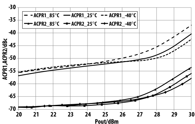
Figure 19. Over-temperature ACPR1, ACPR2 vs. P_{out} @ 2.35 GHz V_{dd}=V_{ddBias}=5.5\text{ V} operating voltage
