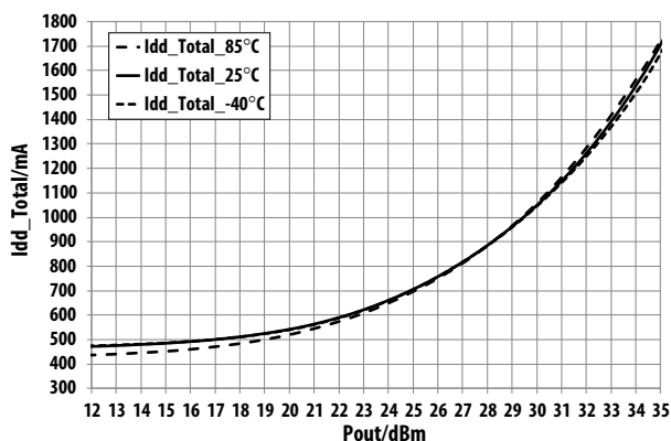
Figure 25. Over-temperature I_{dd\_total} vs. P_{out} @ 2.35 GHz V_{dd}=V_{ddBias}=5.5 V operating voltage
