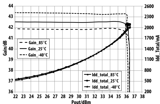
Figure 20. Over-temperature Gain, I_{dd\_total} vs. P_{out} @ 2.33GHz V_{dd}=V_{ddBias}=5.0 V operating voltage
