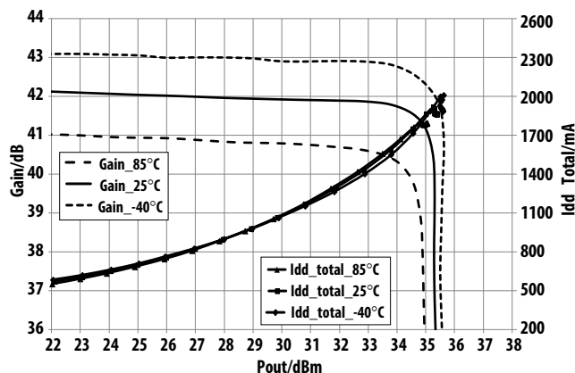
Figure 23. Over-temperature Gain, I_{dd\_total} vs. P_{out} @ 2.39GHz V_{dd}=V_{ddBias}=5.0 V operating voltage
