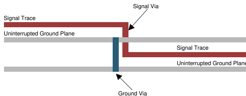
Figure 11-10. Ground Via Location (Side View)
