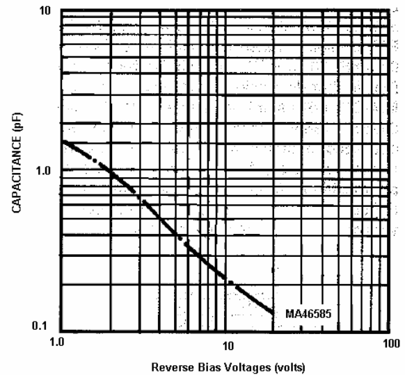
CAPACITANCE vs. VOLTAGE GAMMA = 1.00 +/-10% FROM 2-12V0lts
