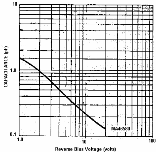
CAPACITANCE vs. VOLTAGE GAMMA = 1.25 +/-10% FROM 2-12V0lts
