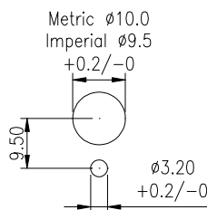
PANEL MOUNTING PIERCING DETAILS
