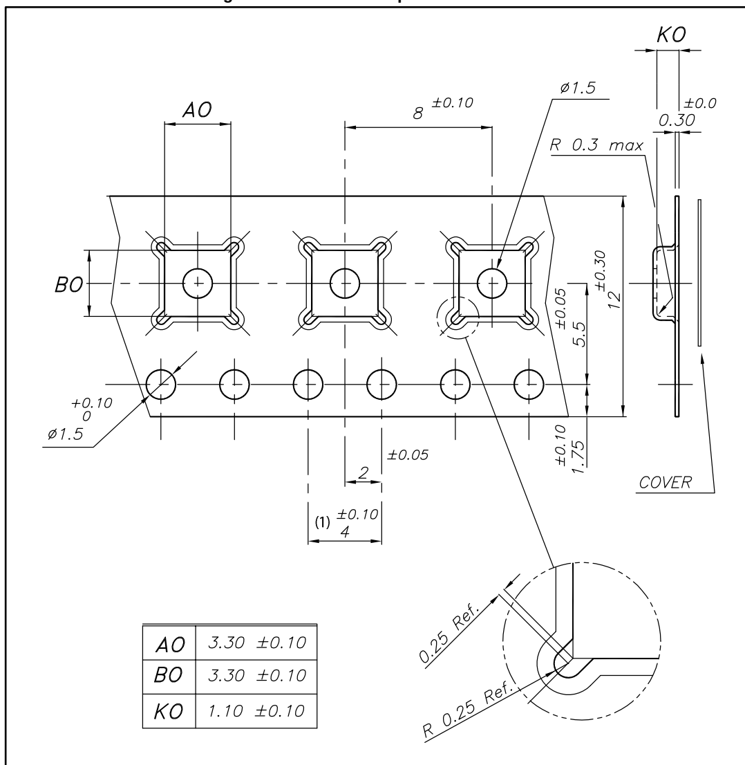
Figure 14: DFN8L 3x3 tape and reel outline
