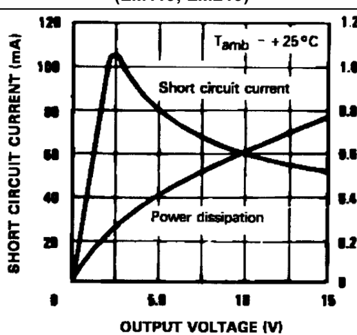
Figure 7. Output limiting characteristics (LM119, LM219)
