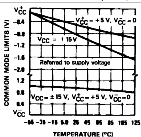
Figure 3. Common mode limits (LM119, LM219)
