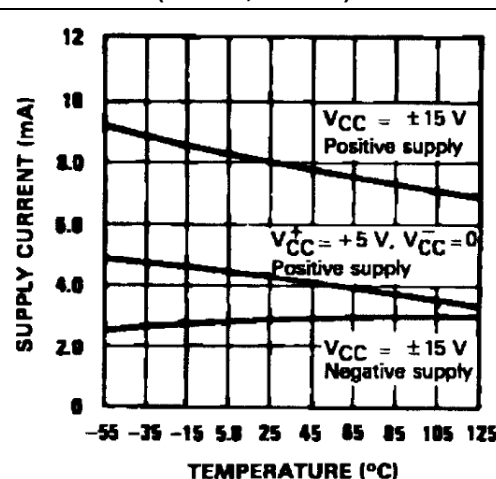
Figure 5. Supply current (LM119, LM219)
