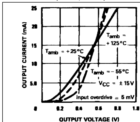
Figure 4. Output saturation voltage (LM119, LM219)
