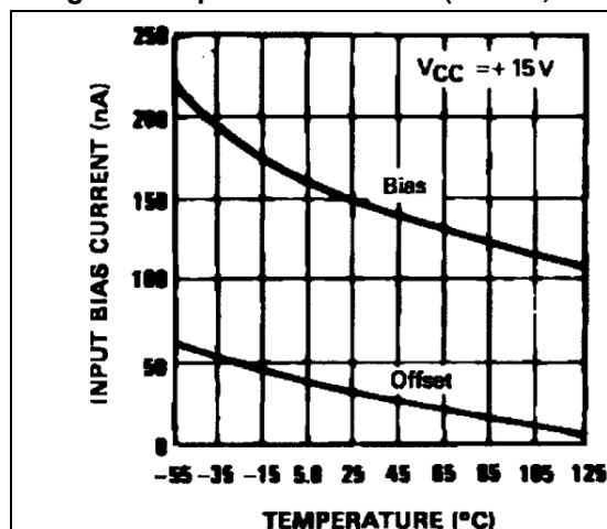
Figure 2. Input bias currents (LM119, LM219)
