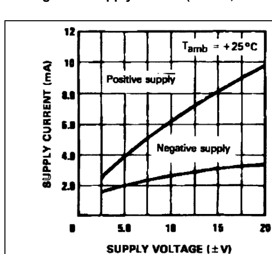
Figure 6. Supply current (LM119, LM219)
