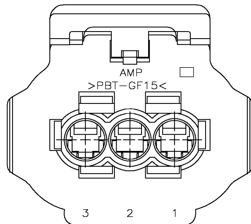
VIEW B-B
