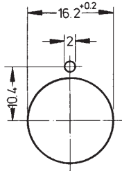
Panel cut-out
