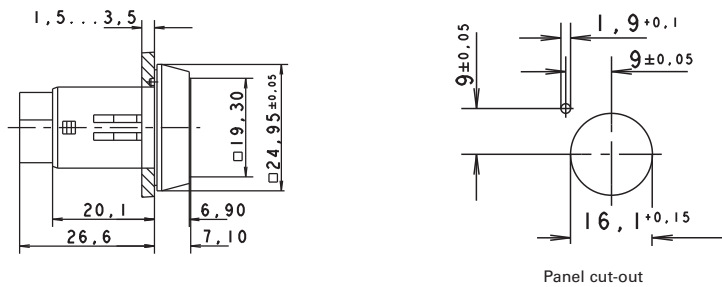
Panel cut-out
