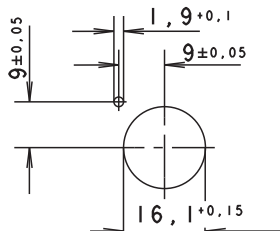
Panel cut-out
