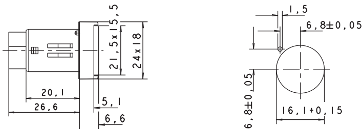
Panel cut-out
