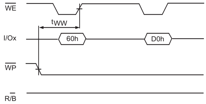
Figure 38 : Disable Erasing
