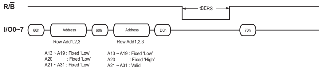
Figure 19 : Multiplane Block Erase
