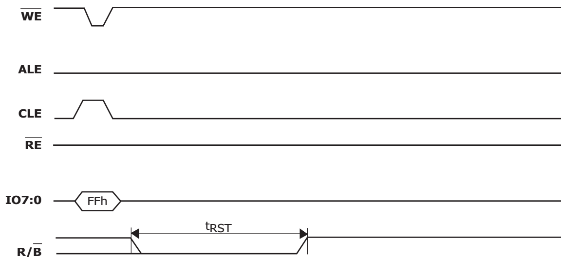
Figure 29 : Reset Operation
