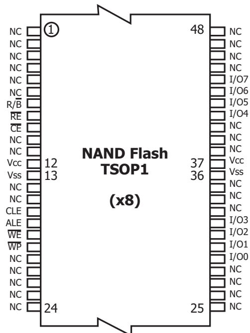
Figure 2 : 48-TSOP1 Contact, x8 Device
