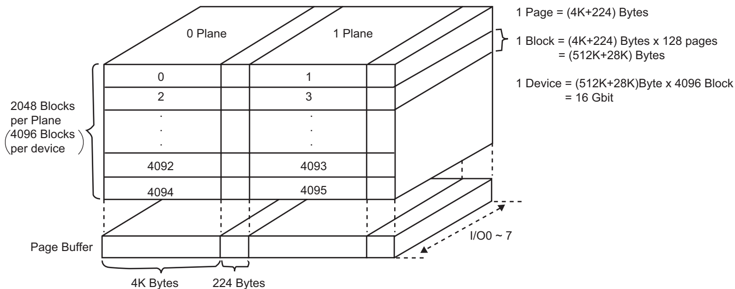
Figure 3 : Array Organization
