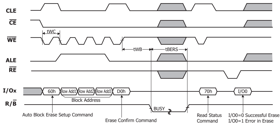
Figure 18 : Block Erase
