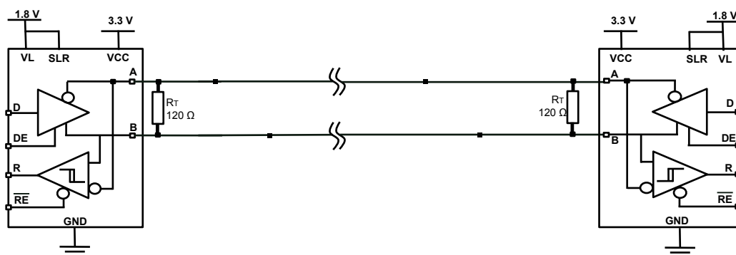
Figure 3. Example of implementation in a PCB
