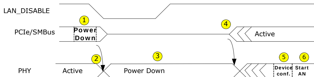
Figure 7. Power-Down Sequence
