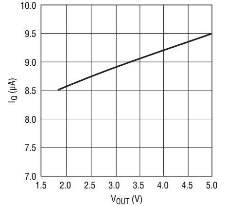
Burst Mode Quiescent Current vs V_{OUT} (LTC3526L)
