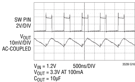
Fixed Frequency Switching Waveform and V_{OUT} Ripple
