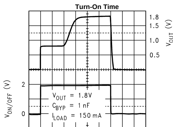
1 ms/div → Figure 33.
