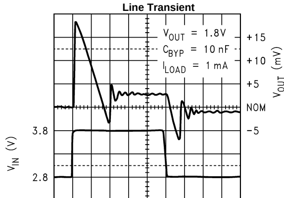
50 \mu\text{s}/\text{div} → Figure 29.
