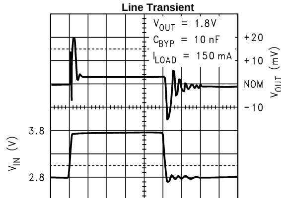
10 \mu\text{s}/\text{div} → Figure 30.
