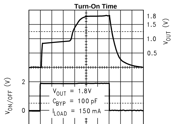
100 \mu\text{s}/\text{div} → Figure 32.
