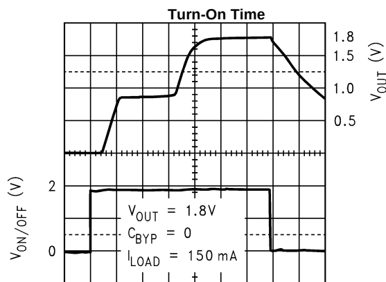
20 \mu\text{s}/\text{div} → Figure 31.
