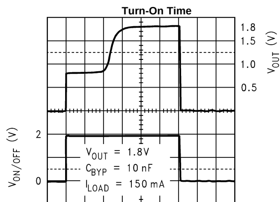
10 ms/div → Figure 34.
