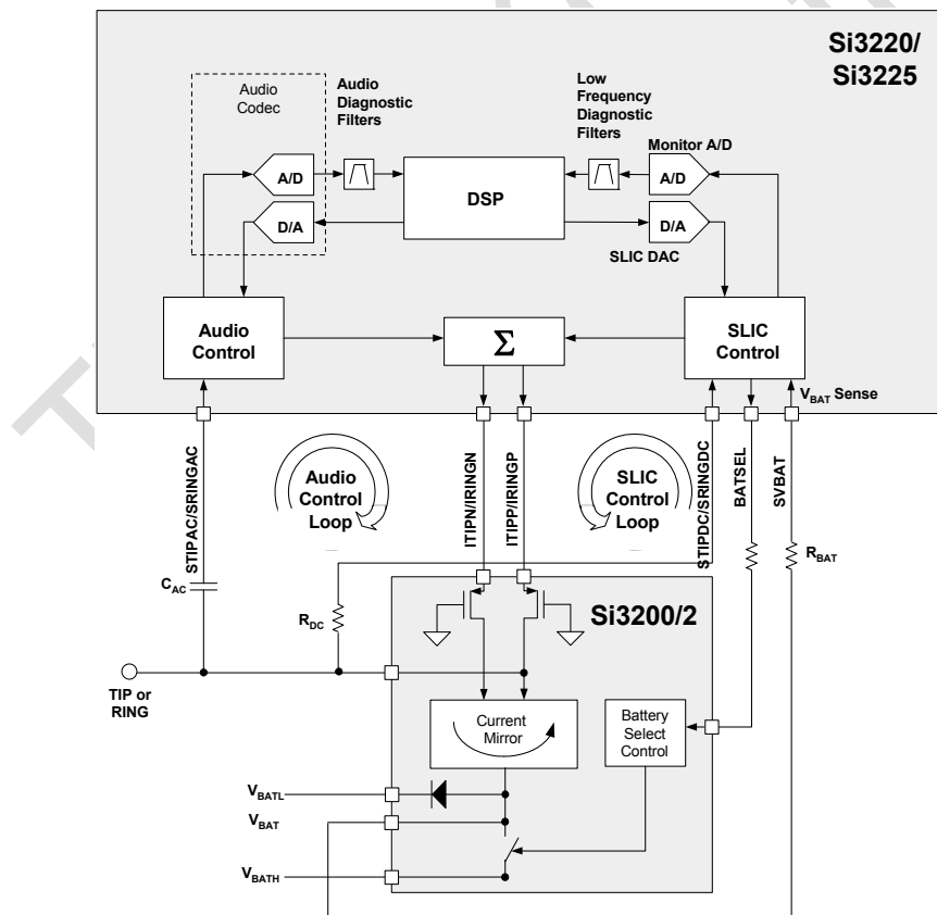
Figure 15. Simplified Dual ProSLIC Linefeed Architecture for TIP and RING Leads (Diagram Illustrates either TIP or RING Lead of a Single Channel)
