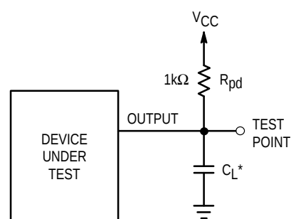
*Includes all probe and jig capacitance
