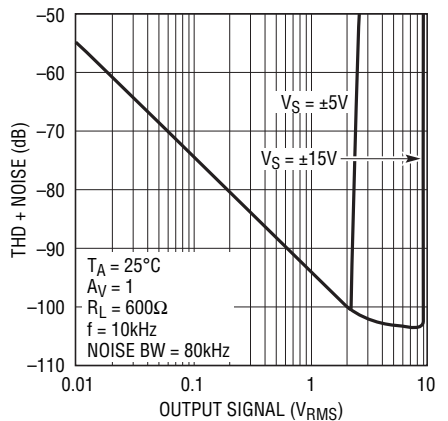
Total Harmonic Distortion + Noise vs Amplitude
