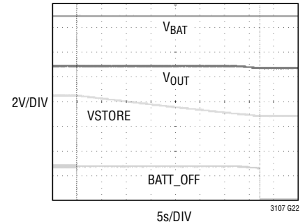
V_{STORE} Holding-Up V_{OUT} ( V_{BAT} = 3V , C_{STORE} = 1300\mu\text{F} , I_{OUT} = 50\mu\text{A} , Holdup = 37 SEC)
