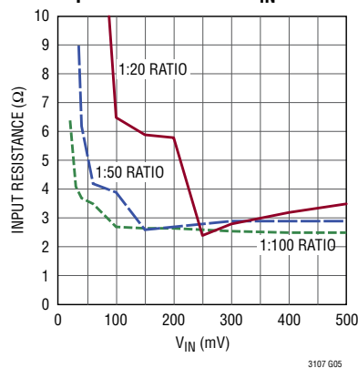
Input Resistance vs V_{IN}
