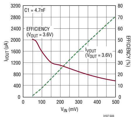
I_{VOUT} and Efficiency vs V_{IN} , 1:50 Ratio Transformer
