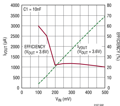
I_{VOUT} and Efficiency vs V_{IN} , 1:20 Ratio Transformer
