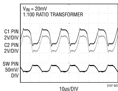
Resonant Switching Waveforms
