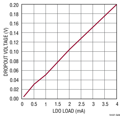
LDO Dropout Voltage
