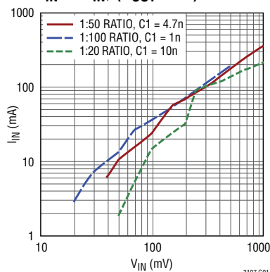
I_{IN} vs V_{IN} , ( V_{OUT} = 0\text{V} )
