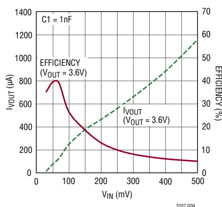
I_{VOUT} and Efficiency vs V_{IN} , 1:100 Ratio Transformer
