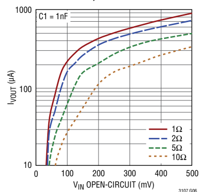
I_{VOUT} vs V_{IN} and Source Resistance, 1:100 Ratio
