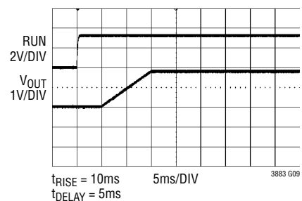
Soft-Start Ramp
