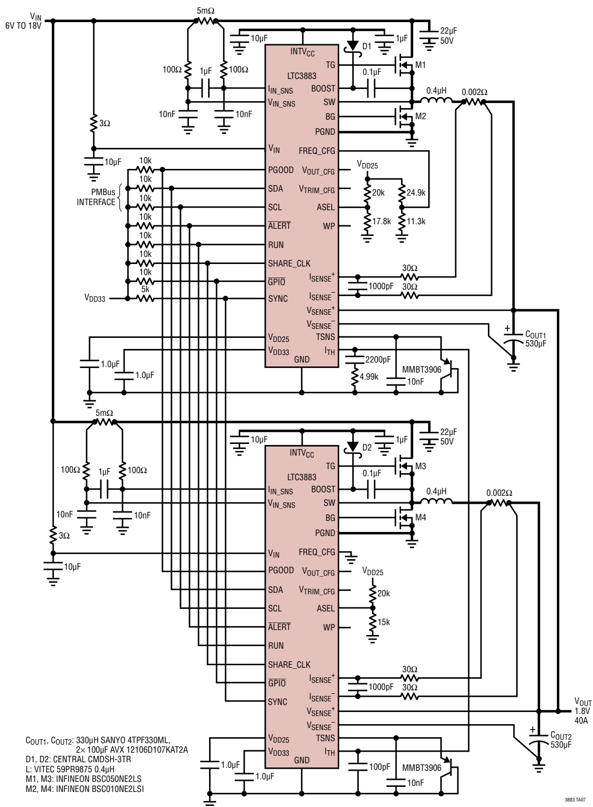
High Efficiency 500kHz 2-Phase 1.8V Step-Down Converter with Sense Resistors
