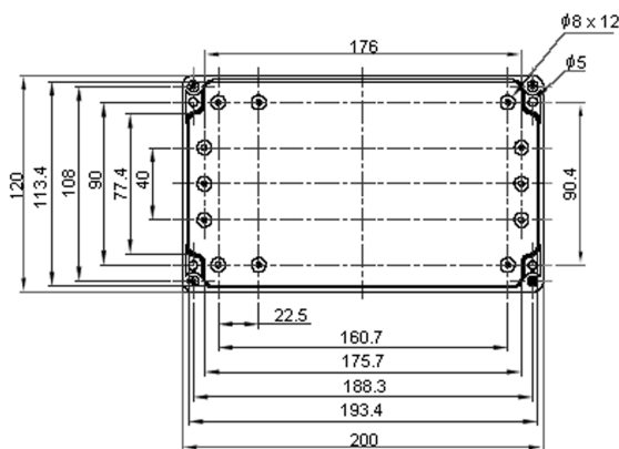
View of Base
