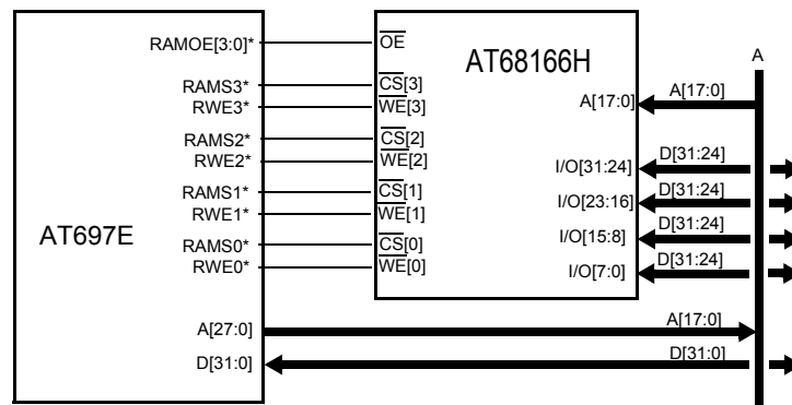
Figure 7. 8-bit typical application (four SRAM banks)
