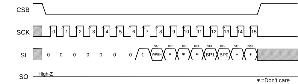
Figure 41. Status register write command
