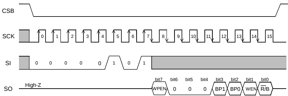
Figure 42. Status register read command
