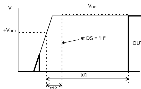
Figure 7 Delay Time
