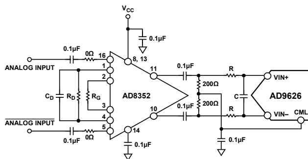
Figure 44. Differential Input Configuration Using the AD8352
