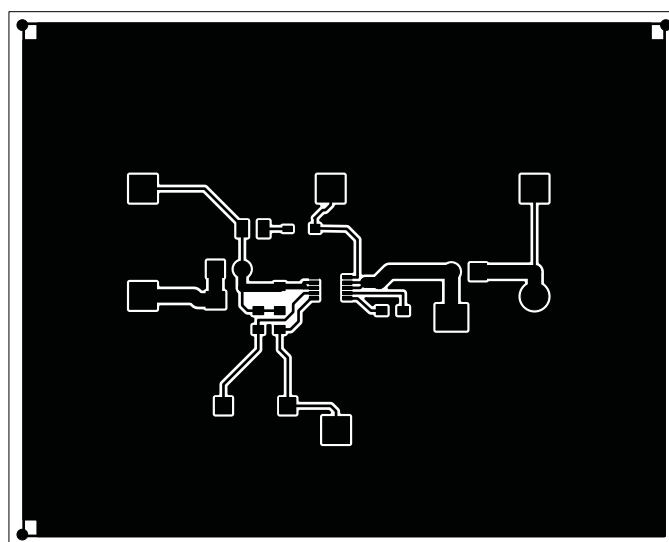
Figure 4. Layer-Two Routing
