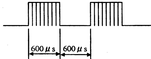
fig. 1 Transmit signal
