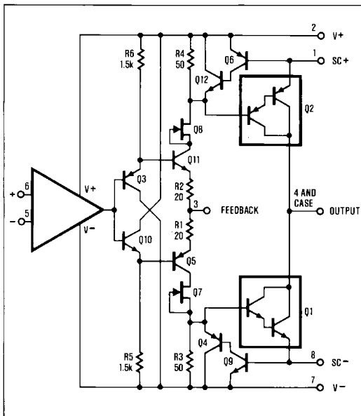
Figure 1. Maxim LH0101 Schematic.
