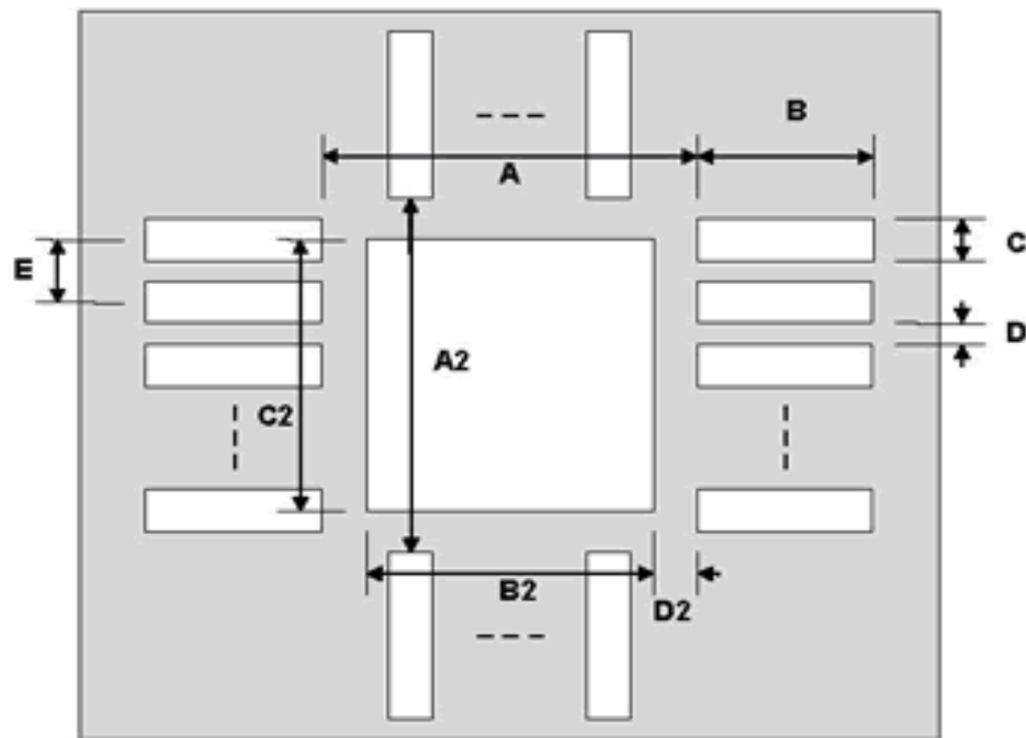
Top View (SMT Footprint)
