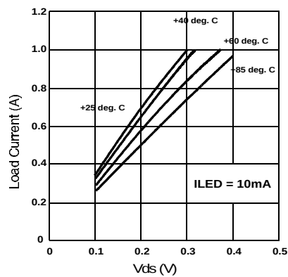
Figure 3. Typical On-Characteristics
