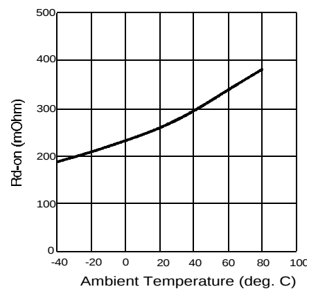
Figure 4. Typical On-Resistance
