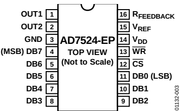
Figure 3. Pin Configuration
