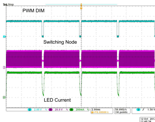
Figure 5-6. PWM Dimming, f_{PWM} = 200 Hz, Duty Cycle = 95%
