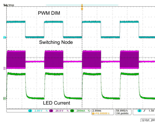
Figure 5-4. PWM Dimming, f_{\text{PWM}} = 200 \text{ Hz} , Duty Cycle = 50%
