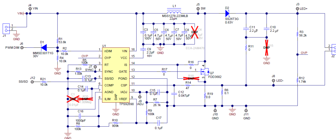
Figure 4-1. TPS92690EVM Schematic
