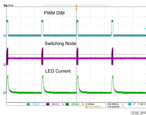
Figure 5-5. PWM Dimming, f_{\text{PWM}} = 200 \text{ Hz} , Duty Cycle = 5%
