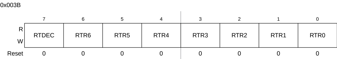
Figure 7-11. S12CPMU RTI Control Register (CPMURTI)
