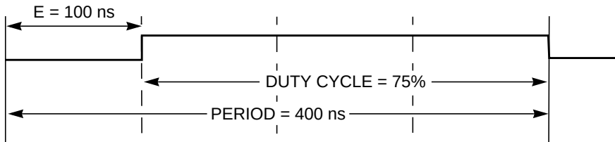
Figure 10-37. PWM Left Aligned Output Example Waveform
