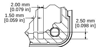
DETAIL L
