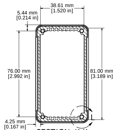
SECTION K-K
