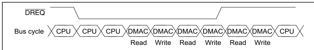
Figure 12.15 Example of Transfer in Burst Mode
