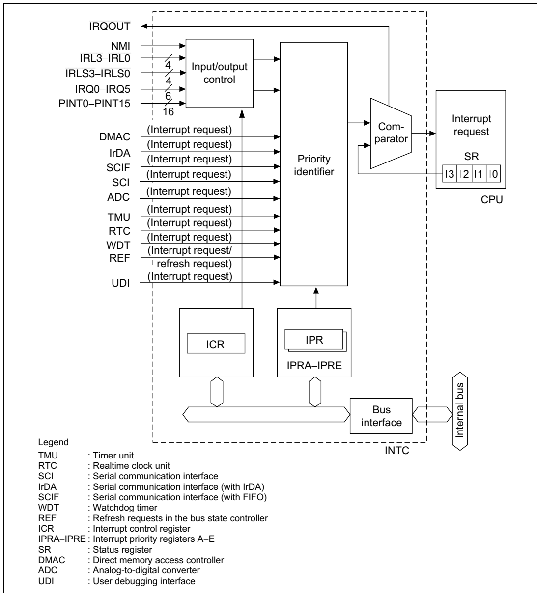
Figure 7.1 Block Diagram of INTIC
