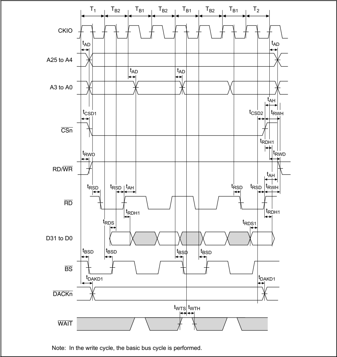
Figure 24.19 Burst ROM Bus Cycle (No Wait)
