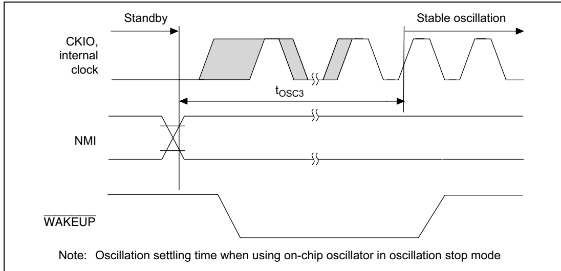
Figure 24.6 Oscillation Settling Time on Return from Standby (Return by NMI)
