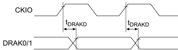
Figure 24.54 \text{DRAK} Output Timing
