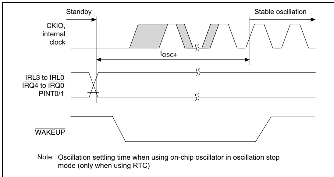
Figure 24.7 Oscillation Settling Time on Return from Standby (Return by \overline{\text{IRQ4}} to \overline{\text{IRQ0}} , \overline{\text{PINT0/1}} and \overline{\text{IRL3}} to \overline{\text{IRL0}} )
