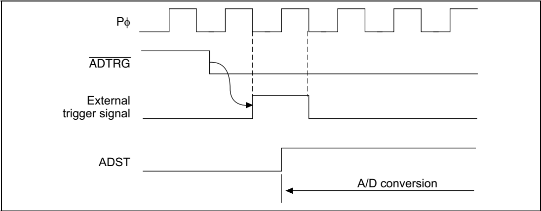
Figure 21.7 External Trigger Input Timing
