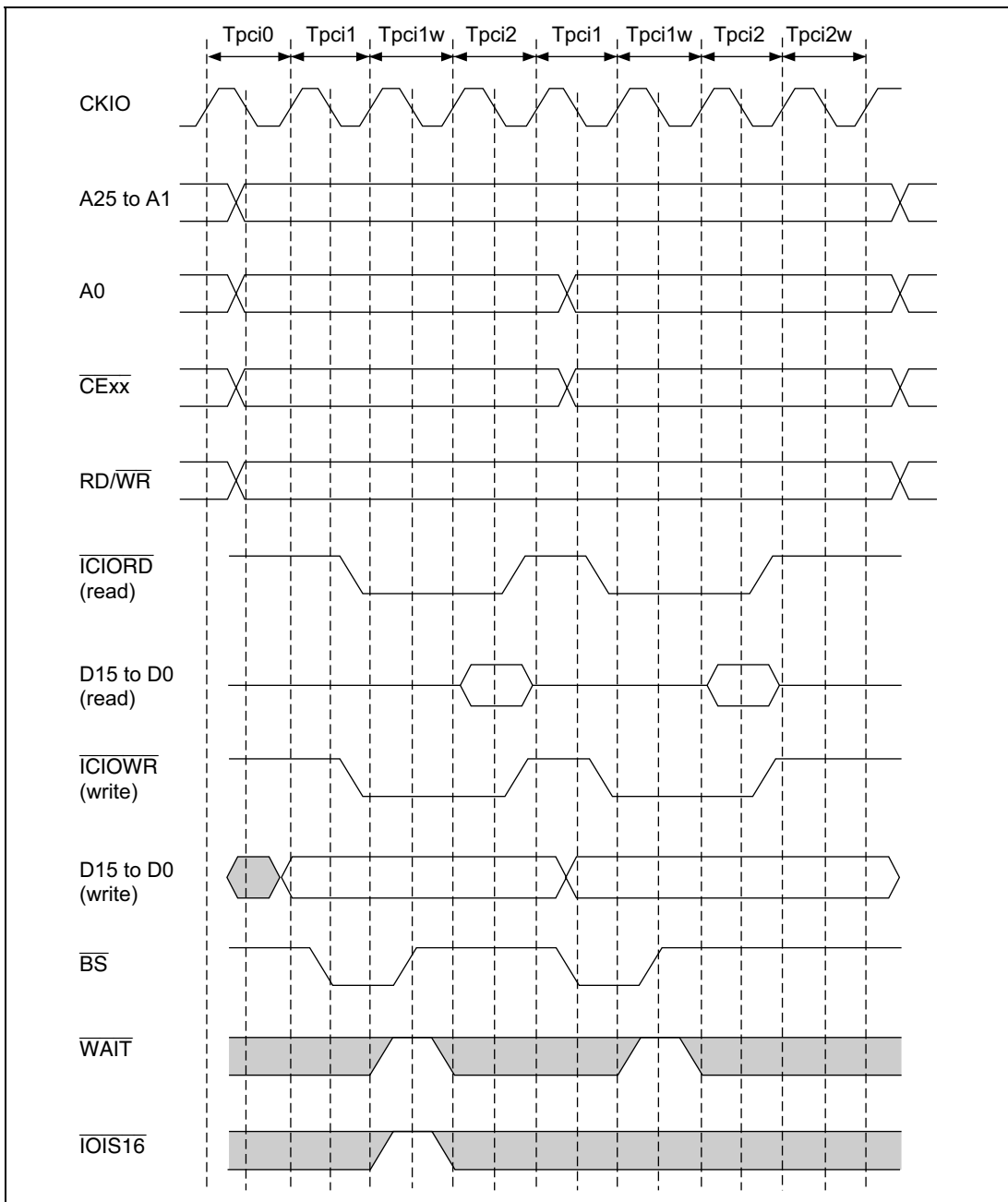
Figure 11.39 Dynamic Bus Sizing Timing for PCMCIA I/O Card Interface
