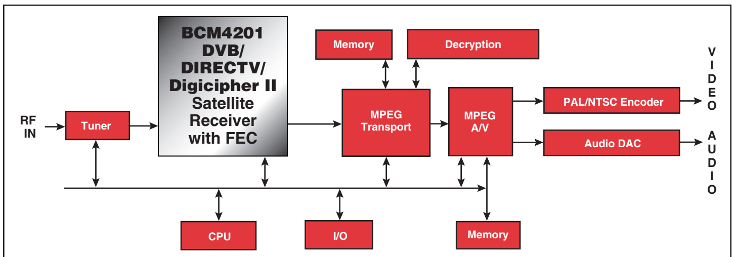
Satellite IRD Block Diagram
